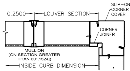
PARTIAL HORIZONTAL SECTION
