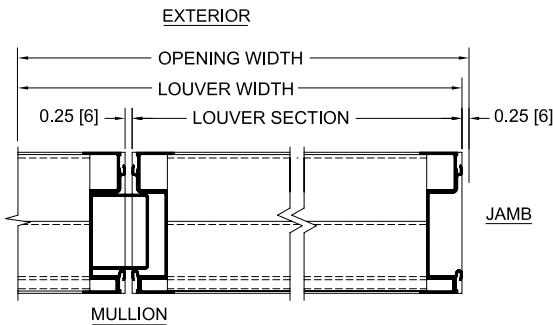
TOP VIEW - HORIZONTAL SECTION
