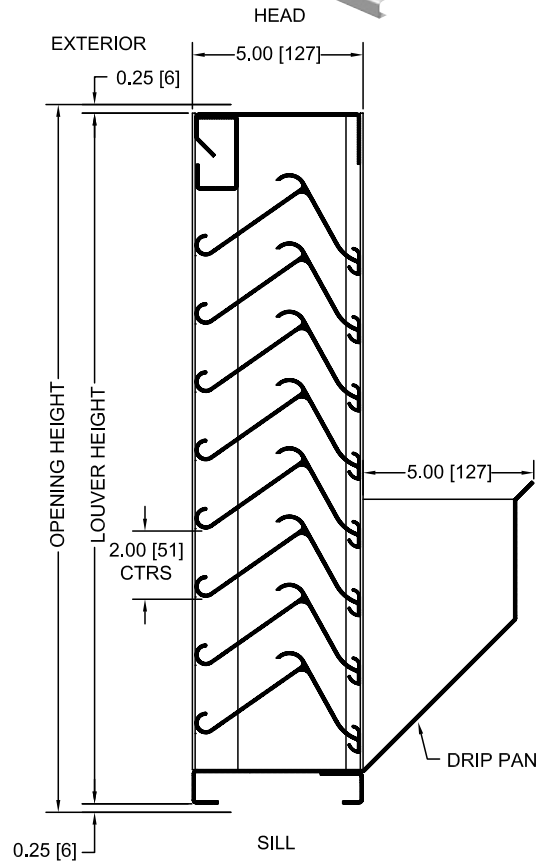
VERTICAL SECTION
